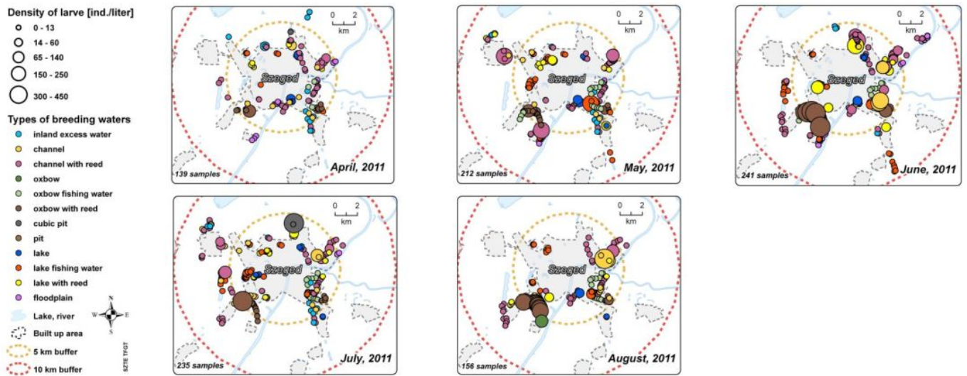
Density of larvae of biting mosquitoes collected in different types of breeding sites in Szeged in 2011
